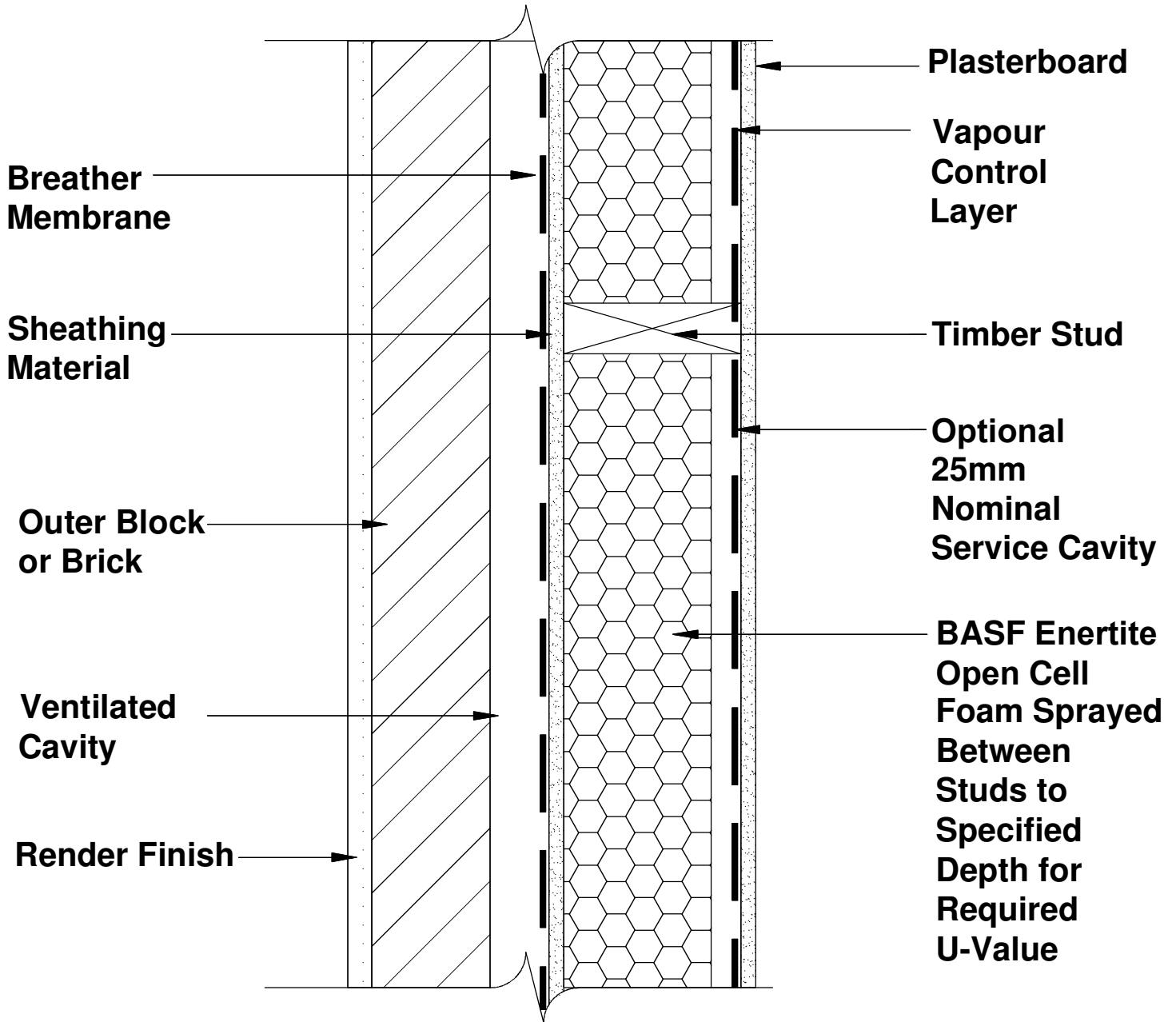
New Build Timber Frame Wall (Plan Section)
