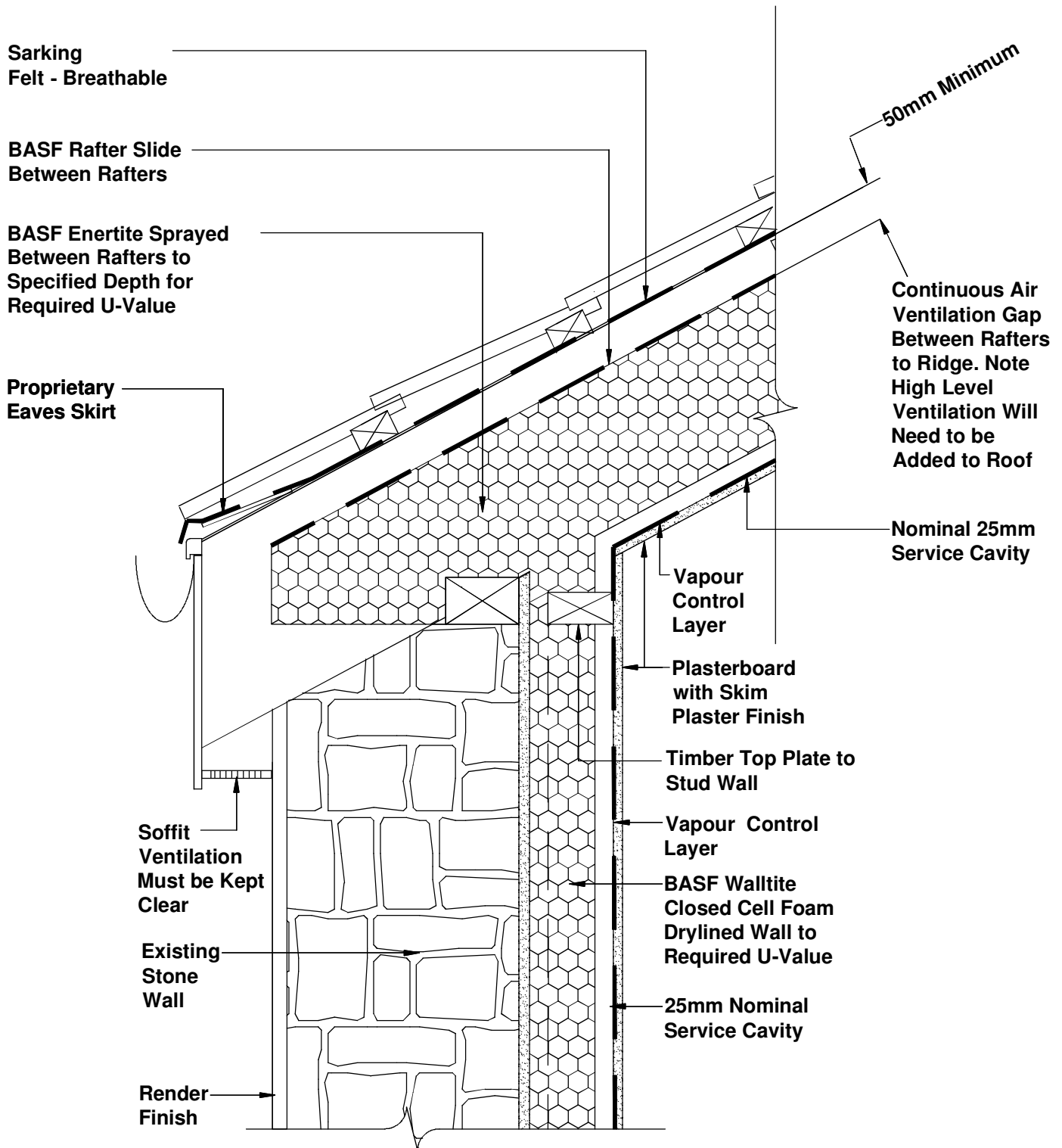
PITCHED ROOF & DRYLINED WALL (INSULATION ON SLOPE BETWEEN RAFTERS)
